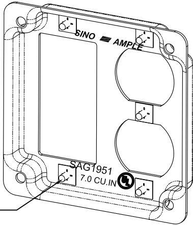
#6-32 UNC,×5
