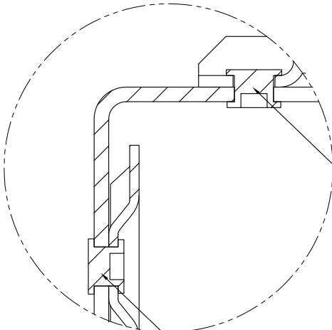
VIEW B
