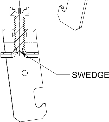
CUTAWAY VIEW A-A
