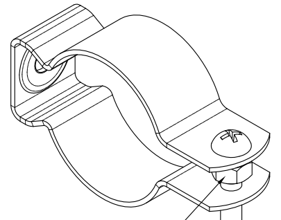
#1/4-20,NUT #1/4-20,SCREW
