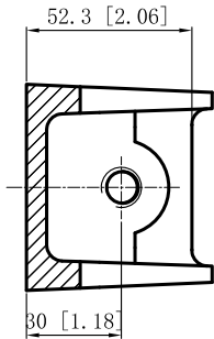
CUTAWAY VIEW B-B
