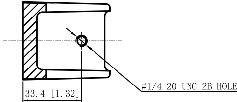
CUTAWAY VIEW B-B
