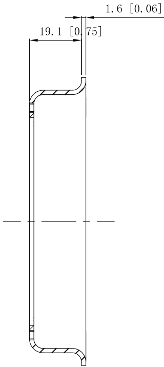
CUTAWAY VIEW A-A
