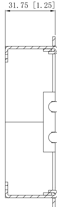
CUTAWAY VIEW A-A
