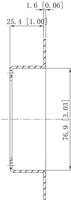
CUTAWAY VIEW A-A
