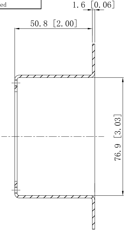
CUTAWAY VIEW A-A
