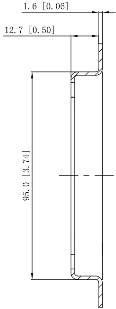
CUTAWAY VIEW B-B
