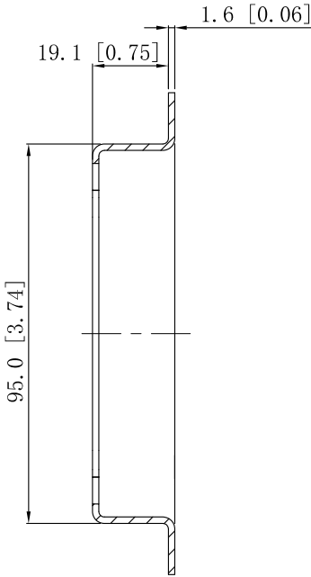
CUTAWAY VIEW B-B
