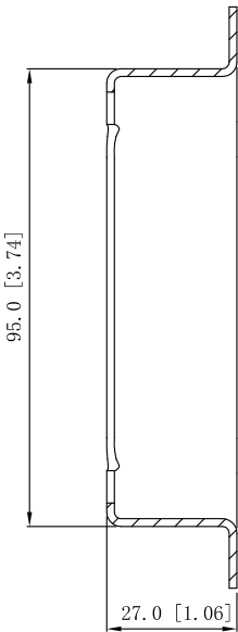
CUTAWAY VIEW B-B
