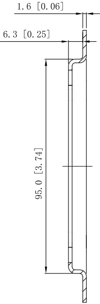
VIEW B-B
