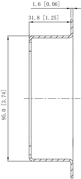
VIEW B-B
