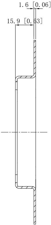
CUTAWAY VIEW A-A
