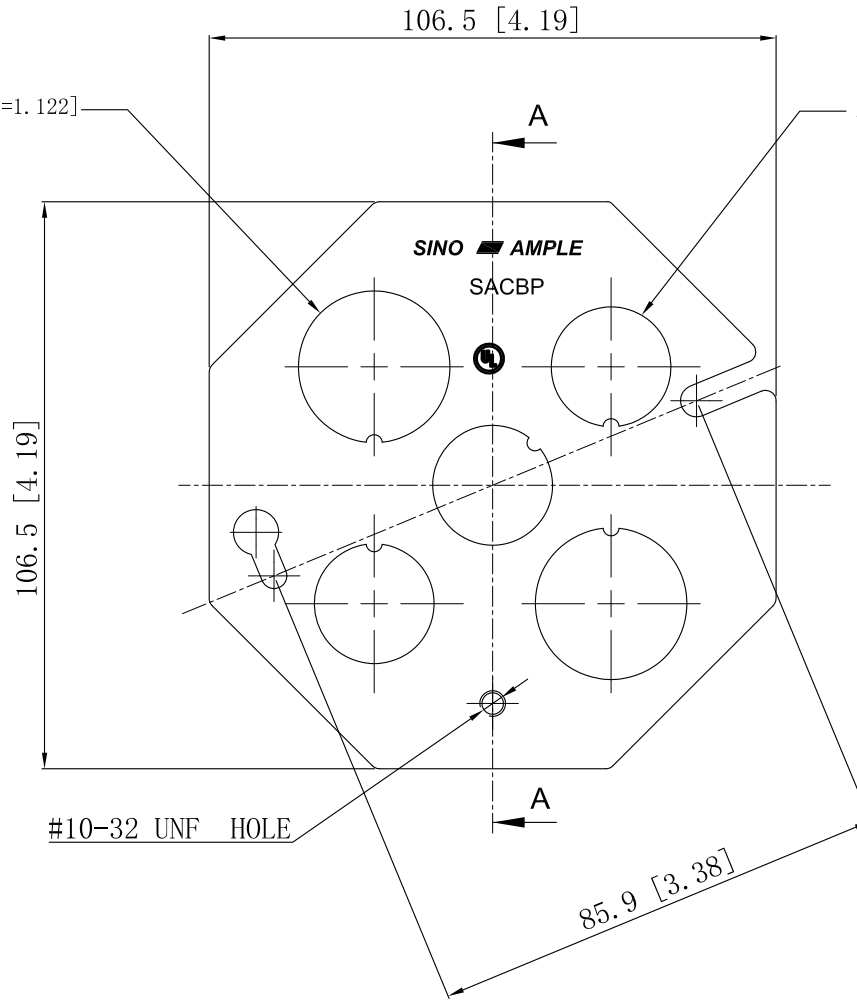
CUTAWAY VIEW A-A
