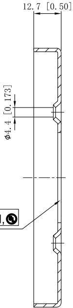
CUTAWAY VIEW A-A
