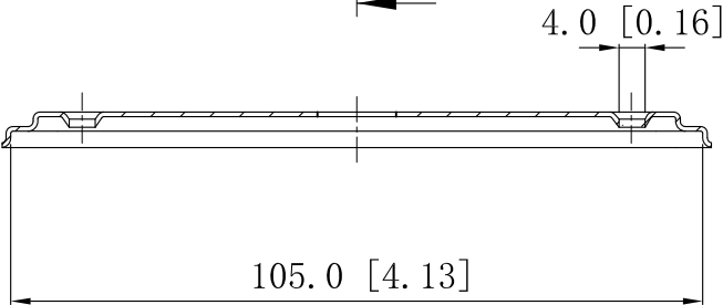
CUTAWAY VIEW B-B
