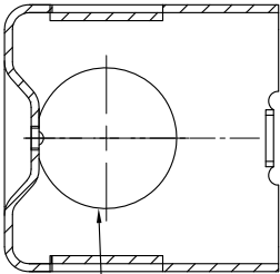
2 3/4"KNOCKOUTS \phi=28.5[\phi=1.12] MIRROR
