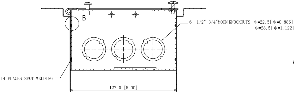
CUTAWAY VIEW A-A
