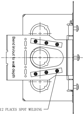
12 PLACES SPOT WELDING
